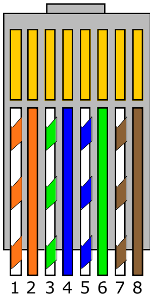
Cross-Connect Cable Termination 1
