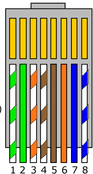
Cross-Connect Cable Termination 2
