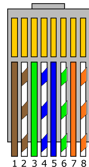
Rollover Cable Termination 2
