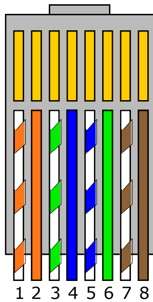
Standard Patch Cable Termination 1 & 2 (Same) EIA/TIA-568-A Pinout for T568B
